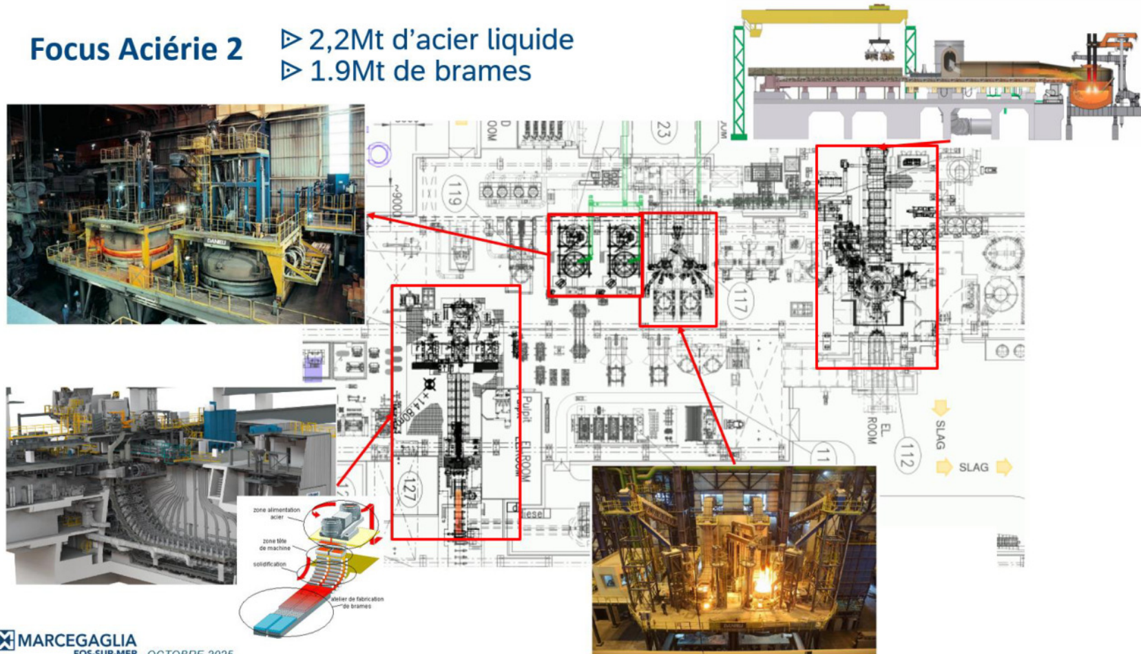
Figure 43: Plan Aciérie
