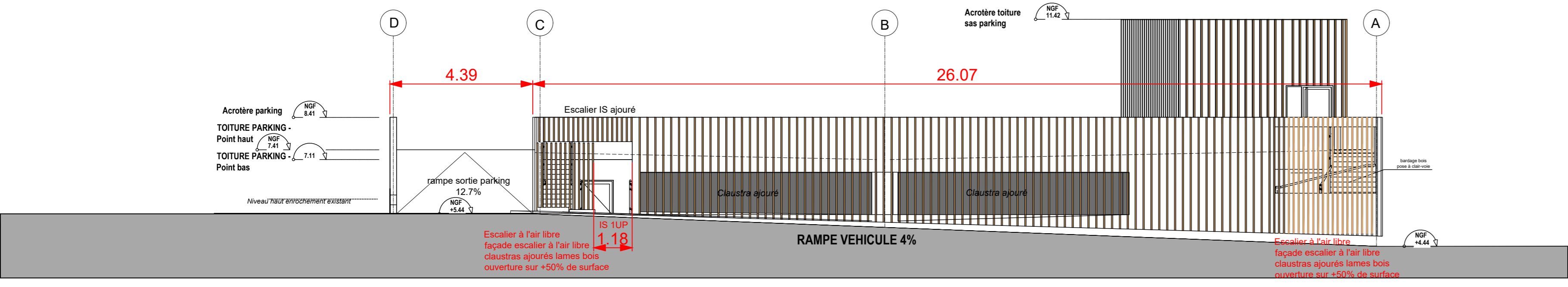
FACADE NORD-EST Parking silo
