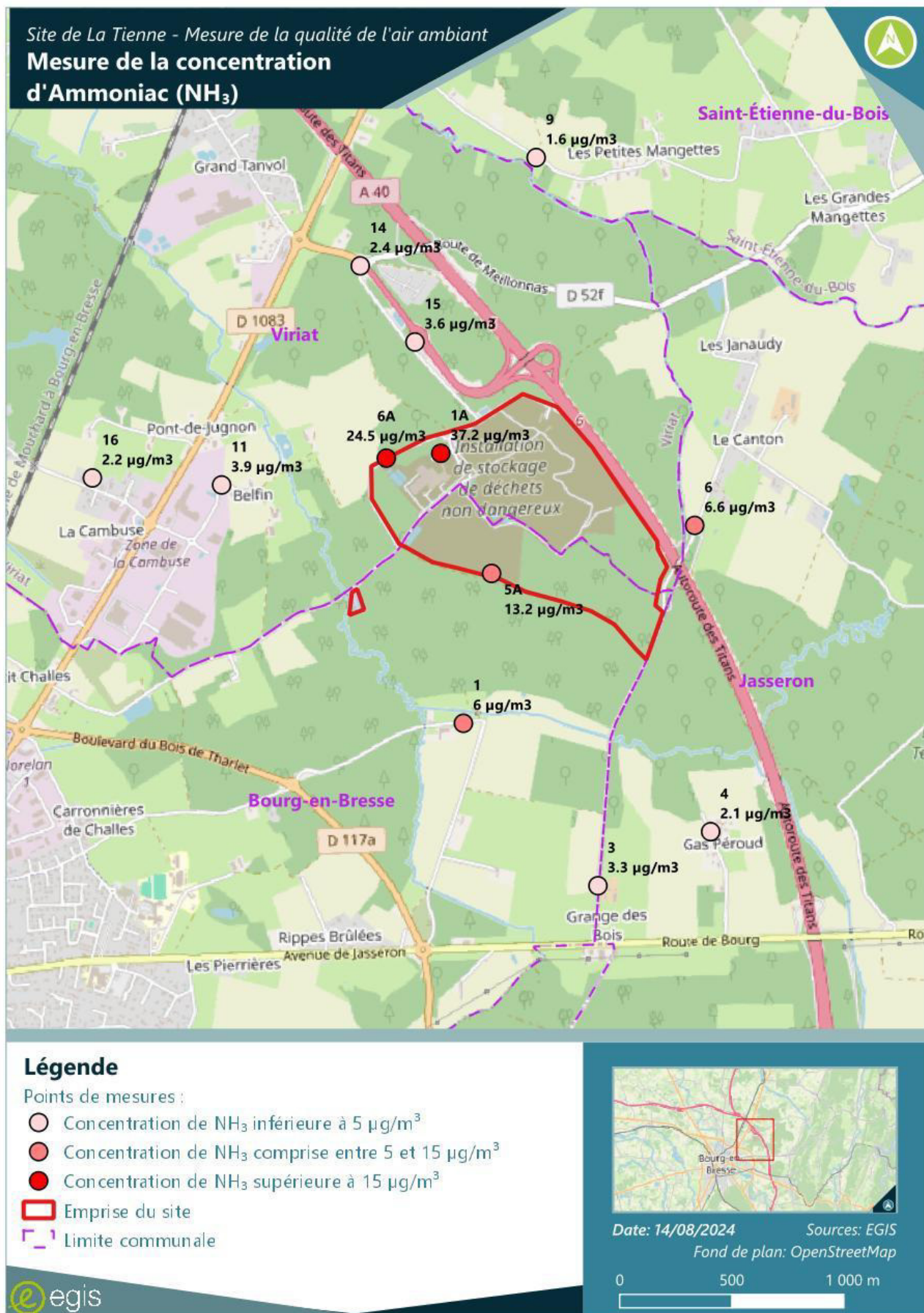
FIGURE 6 : CONCENTRATION EN AMMONIAC ( \text{NH}_3 ) EN \mu\text{g}/\text{m}^3 .
