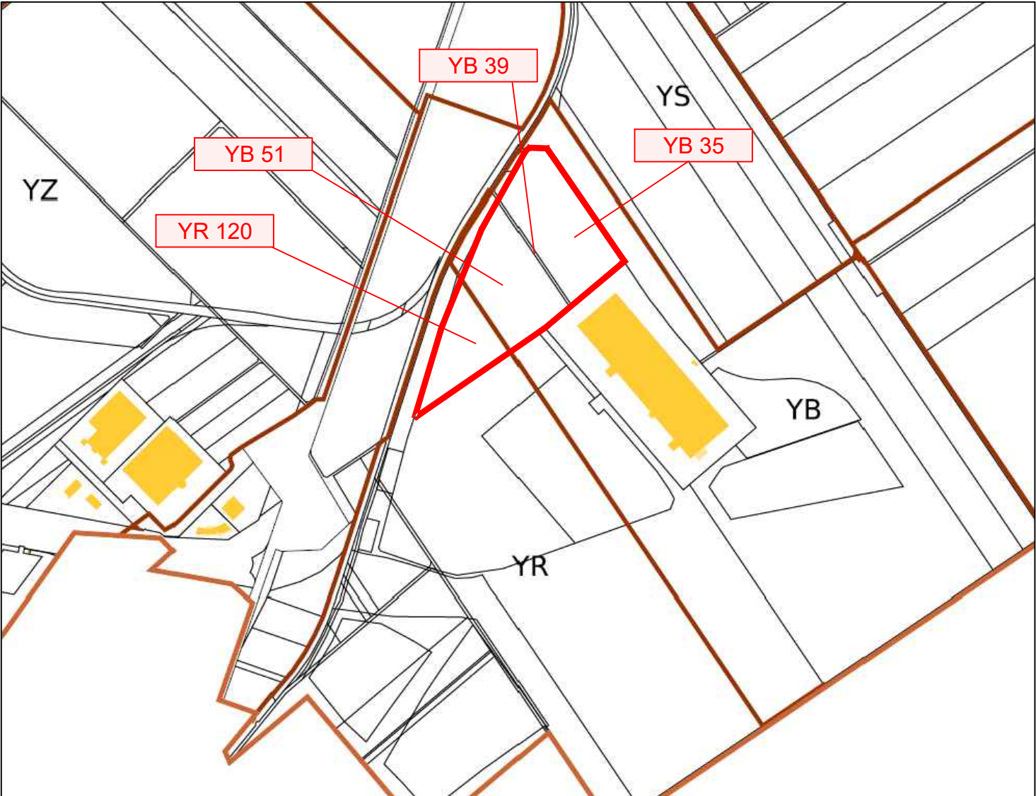
PLAN CADASTRAL
