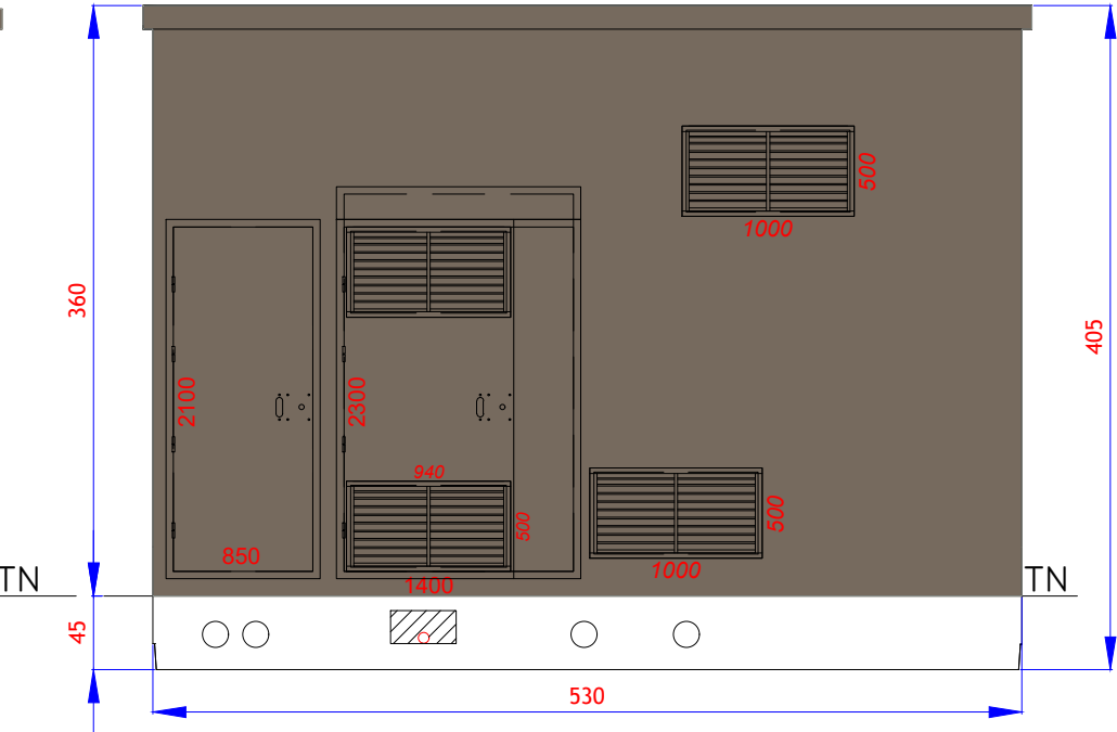
FAÇADE ARRIERE
